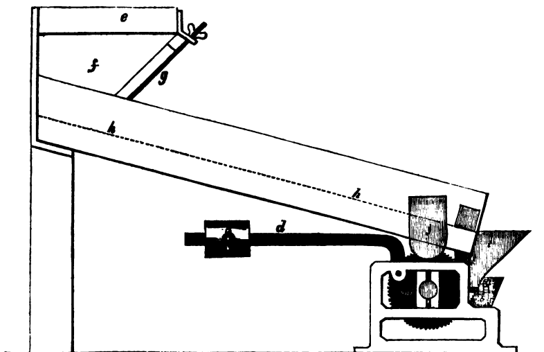
WILLIAMS' MALT GRINDER.
